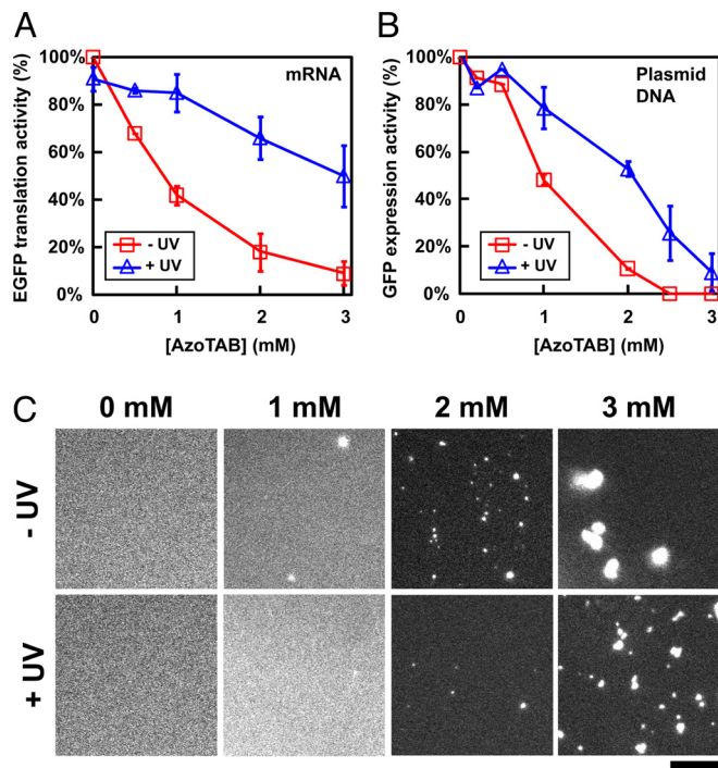
Fig. 4. Translation and expression of a fluorescent protein is photocontrolled using AzoTAB in a cell-free expression system. (A) Translation activity of a mRNA coding for EGFP and (B) expression activity of a plasmid coding for GFP protein as a function of AzoTAB concentration in the absence (red squares) and in the presence (blue triangles) of 1.5 min of 365 nm UV illumination. The experiments were performed in PURE System, with mRNA and DNA templates both at a final concentration of 1 \mu\text{g}/\text{mL} . (C) Representative fluorescence microscopy images of mRNA (50 nM) labeled by Ribogreen in PURE System buffer without tRNA and protein factors as a function of AzoTAB concentration, with or without UV exposure (365 nm). Images were focused on the glass substrate. (Scale bar, 10 \mu\text{m} .)
