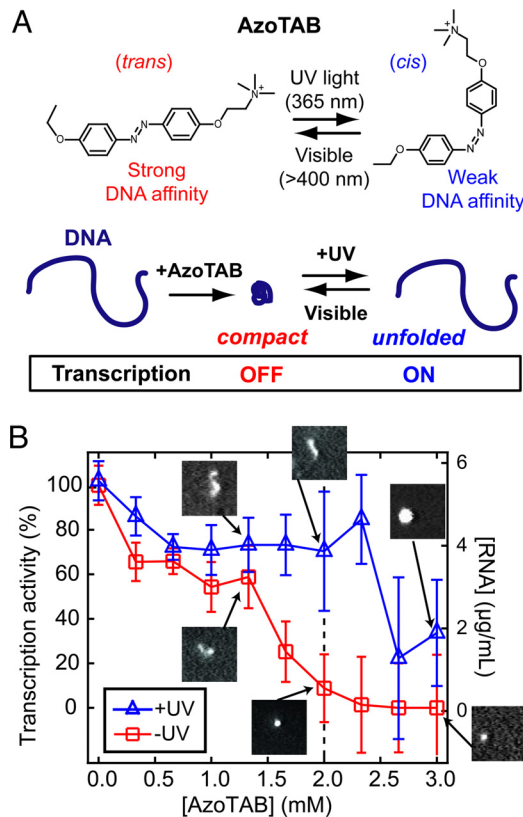
Fig. 1. The conformation and transcription activity of genomic DNA is controlled using UV illumination in the presence of the photosensitive condensing agent AzoTAB. (A) After addition of trans -AzoTAB, DNA is compact and transcription is inhibited. Upon UV illumination, AzoTAB isomerizes to cis , which triggers DNA unfolding and switches on transcription. The process is reversible upon VIS (>400 nm) illumination which compacts DNA and switches transcription back to the off state. (B) Transcription activity of T4 DNA as a function of AzoTAB concentration in the dark (red squares) and after UV illumination for 10 min (blue triangles). The Insets show representative fluorescence microscopy images of T4 DNA for 1.3, 2.0, and 3.0 mM AzoTAB demonstrating a good correlation between DNA condensation state and transcription activity. Each image is 6 \times 6 \mu\text{m} . The dashed line represents the onset of increase of static light scattering intensity (-UV) (Fig. S1). All experiments were performed under the same conditions: 1 \mu\text{g/mL} T4 DNA, 0.02 U/ \mu\text{L} E. coli RNA polymerase, 40 mM Tris-HCl, pH 7.5, 150 mM KCl, 10 mM \text{MgCl}_2 , 0.5 mM NTPs, and 10 mM DTT, T = 37^\circ\text{C} .
